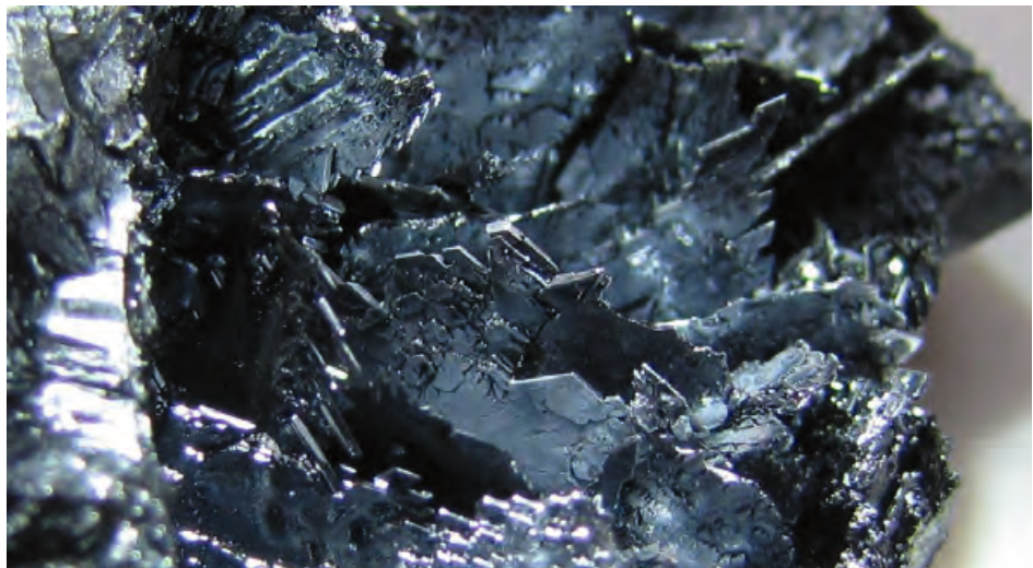
Iodine crystals
